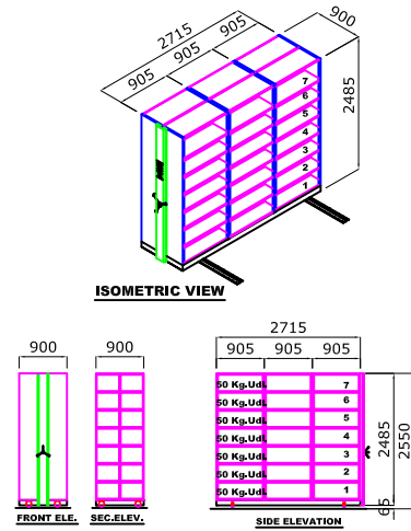
ELEVATION FOR SYSTEM - 2
