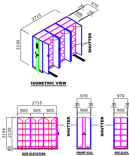
ELEVATION FOR SYSTEM - 1
