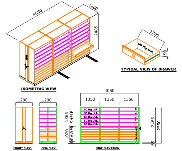
ELEVATION FOR SYSTEM - 3
